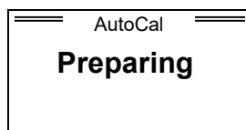
Purging
