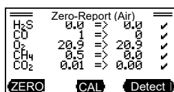
Result of sensor calibration with fresh air (CO 2 -free) Reading before => after
