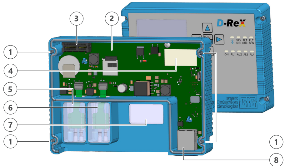
D-ReX housing cover interior view, with LIM
